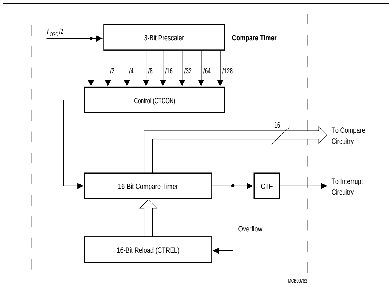
Figure 6-16 Compare Timer Block Diagram
