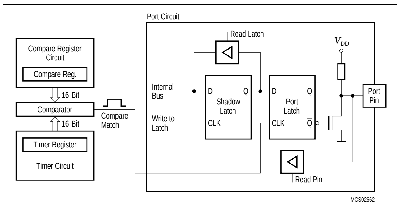
Figure 6-19 Compare Function of Compare Mode 1
