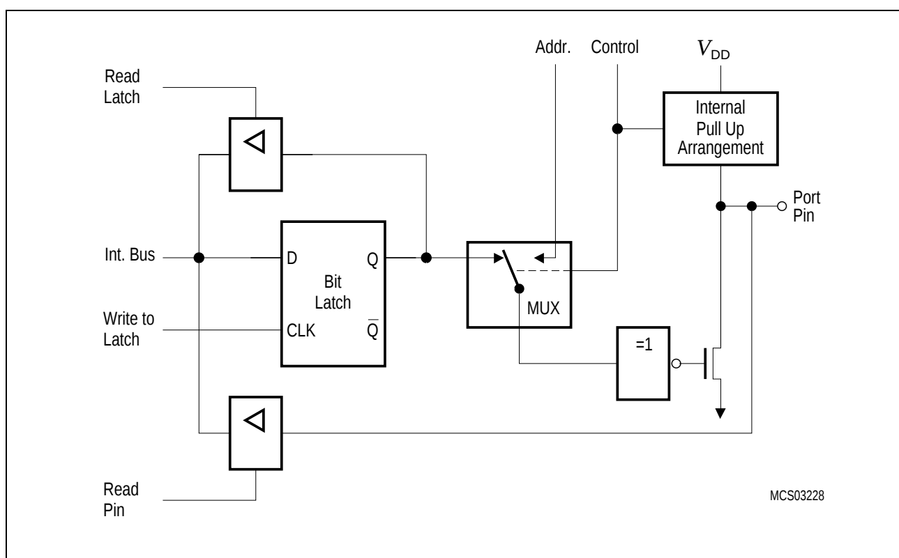
Figure 6-5 Port 2 Circuitry
