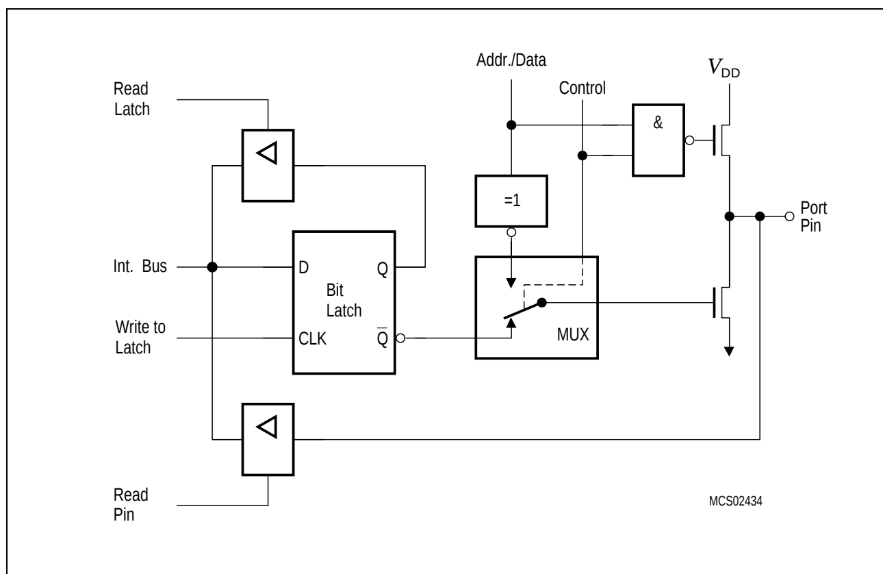
Figure 6-3 Port 0 Circuitry
