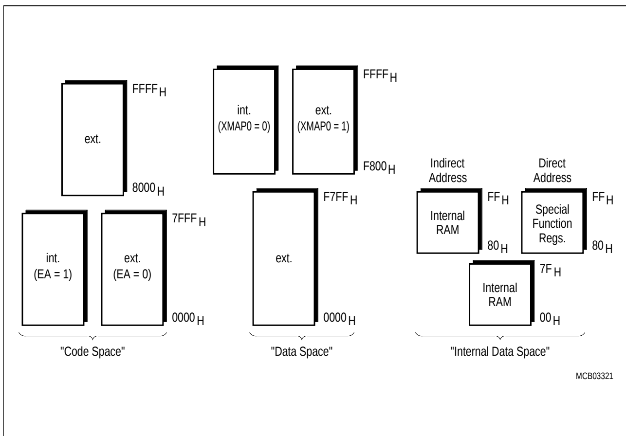
Figure 3-1 C517A Memory Map
