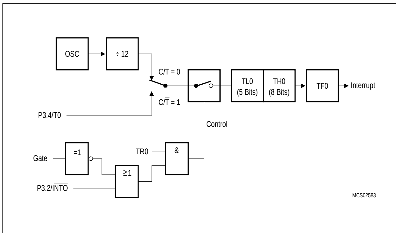
Figure 6-9 Timer/Counter 0, Mode 0: 13-Bit Timer/Counter
