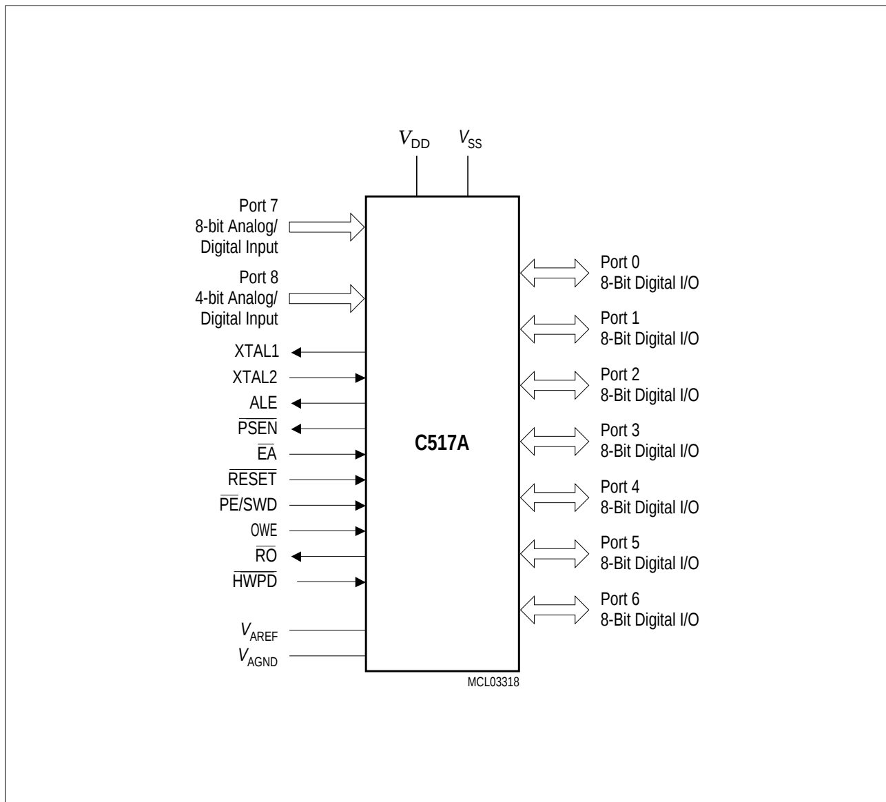
Figure 1-2 Logic Symbol
